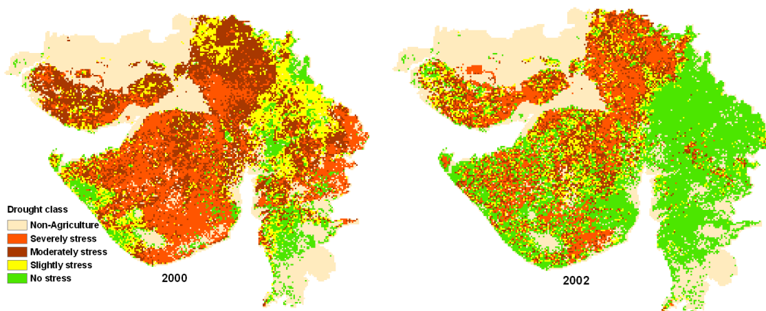
Figure 5.11: Map showing the spatial pattern of drought on 257 JD during 2000 and 2002 based on WDI
