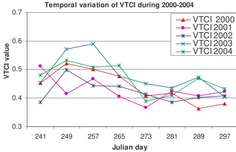
Figure 5.10: The temporal variation of average VTCI curve for Gujarat state during September to October month for 2000-2004
