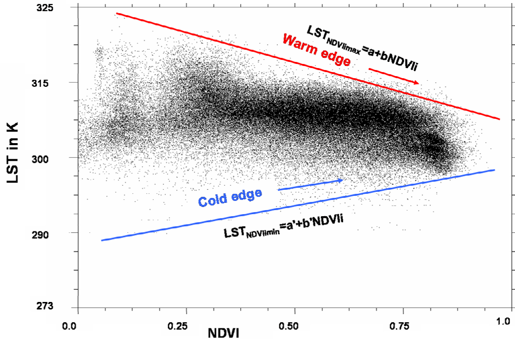
Figure 4.6: Schematic scatter plot of the physical interpretation of VTCI
