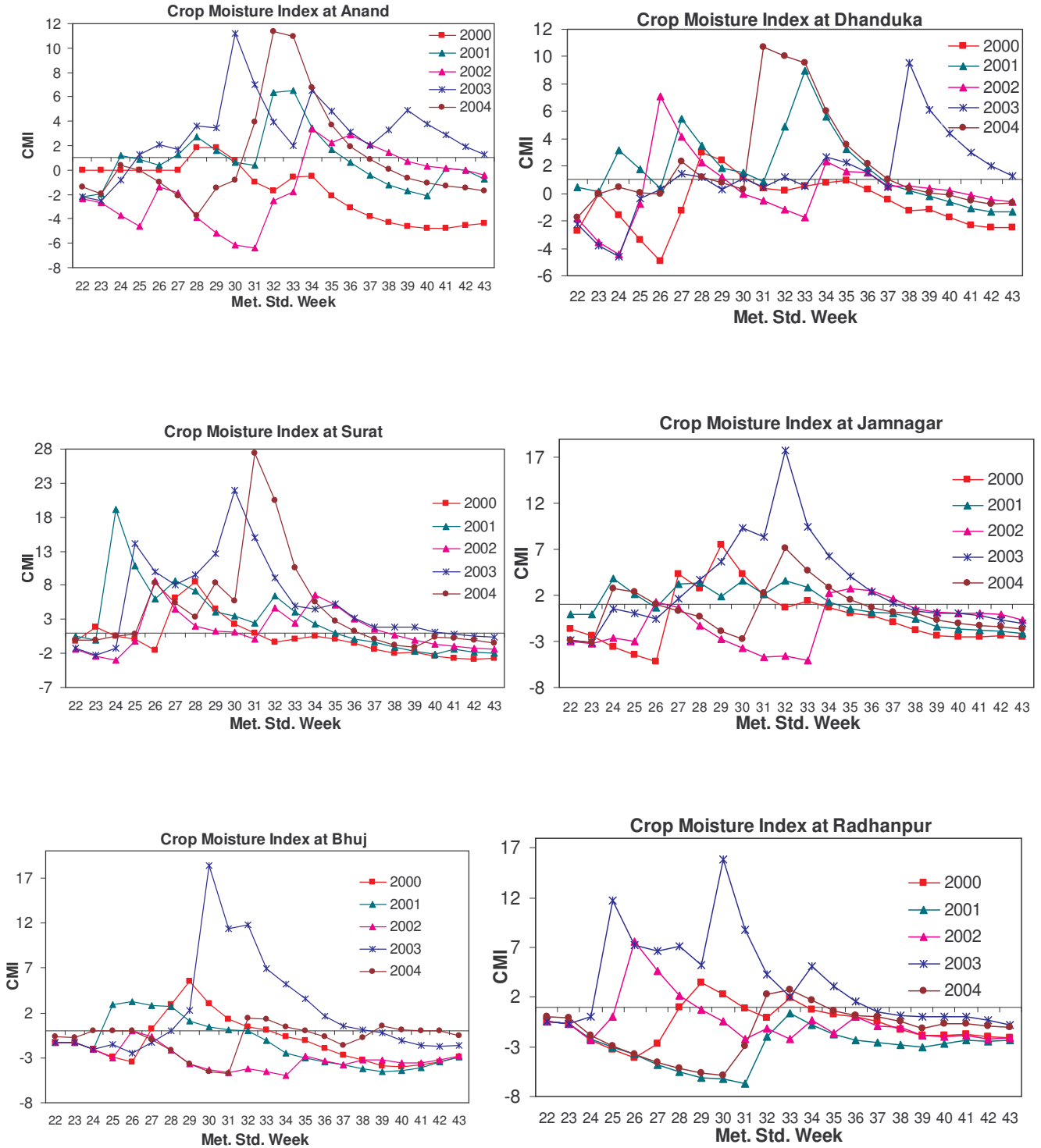
Figure 5.7: The crop moisture index at different stations during 2000 to 2004
