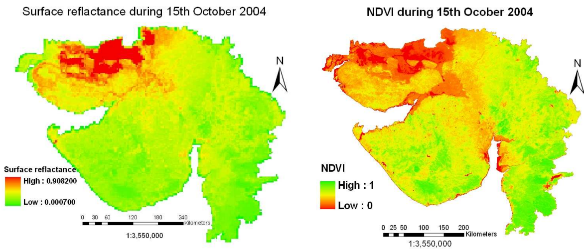
Figure 4.2: The Surface reflectance and NDVI during 15 th October 2004
