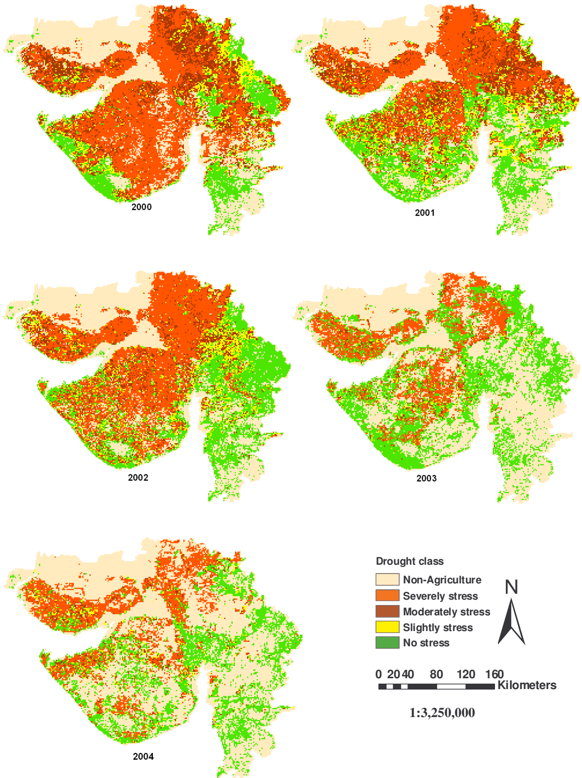
Figure 5.9: Map showing the spatial pattern of drought severity on 257 JD during 2000 to 2004 based on VTCI
