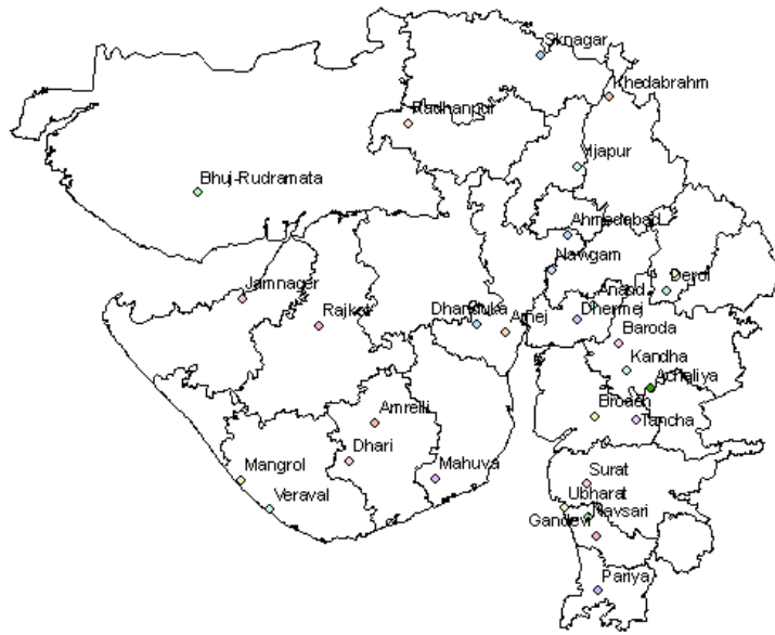
Figure 4.3: The stations used for ambient air temperature interpolation using spline technique
