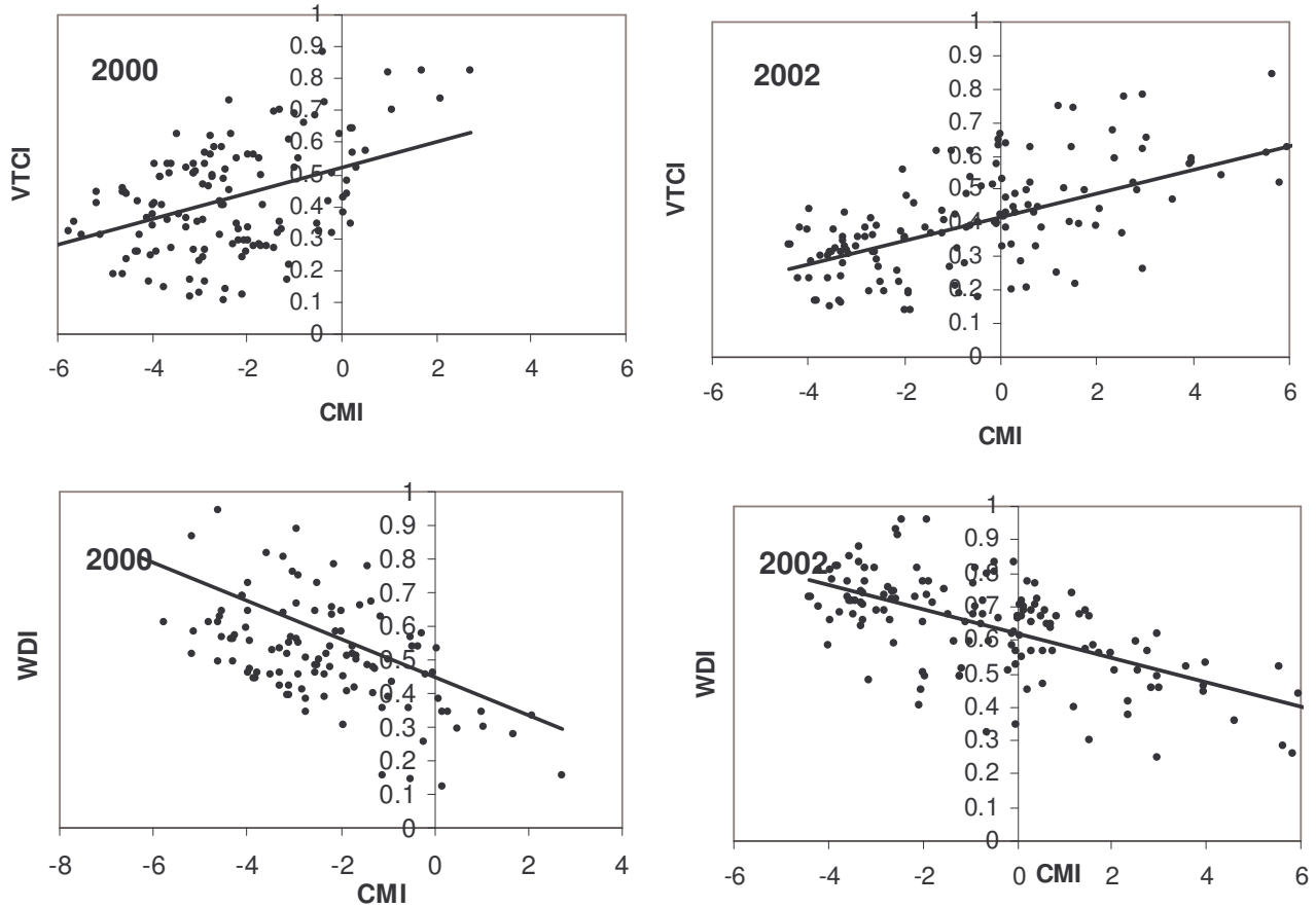
Figure 5.6: The linear regression trend for VTCI and WDI for defining threshold for drought stress
