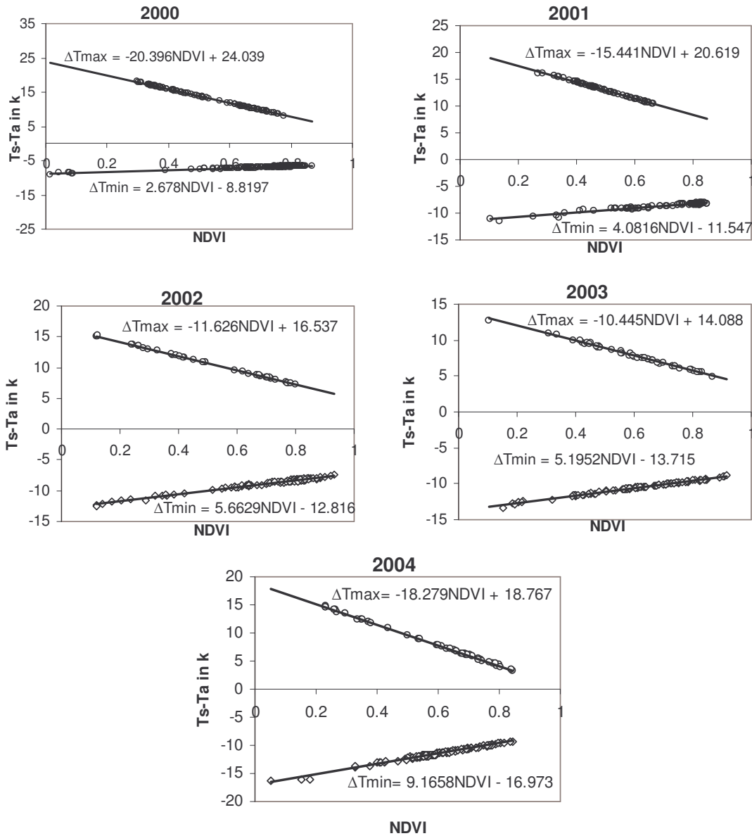
Figure 5.2: The wet line and dry line from NDVI- \Delta T_s space on 257JD
