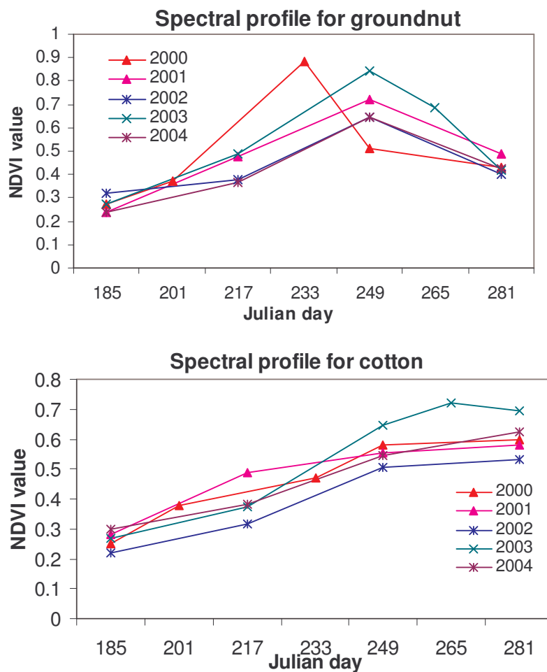
Figure 4.9: The spectral profiles for groundnut and cotton in different years
