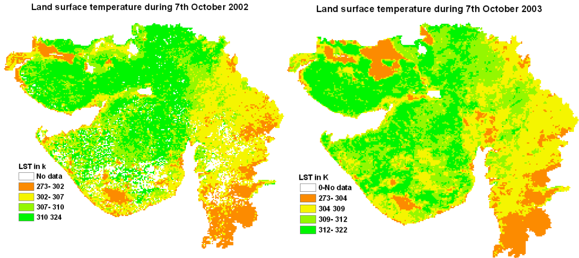
Figure 4.1: The Land surface temperature in different year
