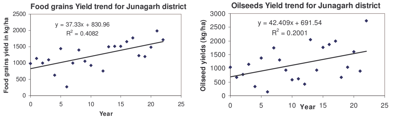
Figure 4.11: The linear regression trend for food grain yield and oilseeds yield
