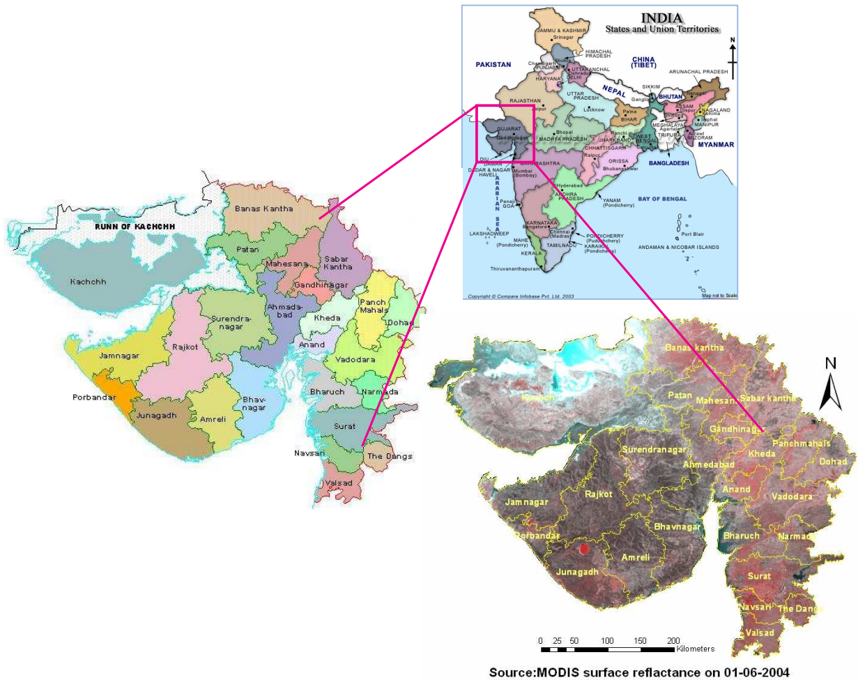
Figure 3.1: The location of study area "Gujarat state" in India
