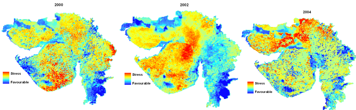
Figure 5.4: Spatial pattern of WDI on 249 JD during 2000, 2002 and 2004 in Gujarat state
