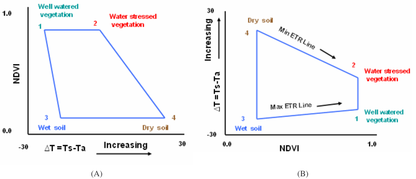
Figure 4.7: The Schematic plot for WDI (Moran, 1994) and modified schematic plot of WDI
