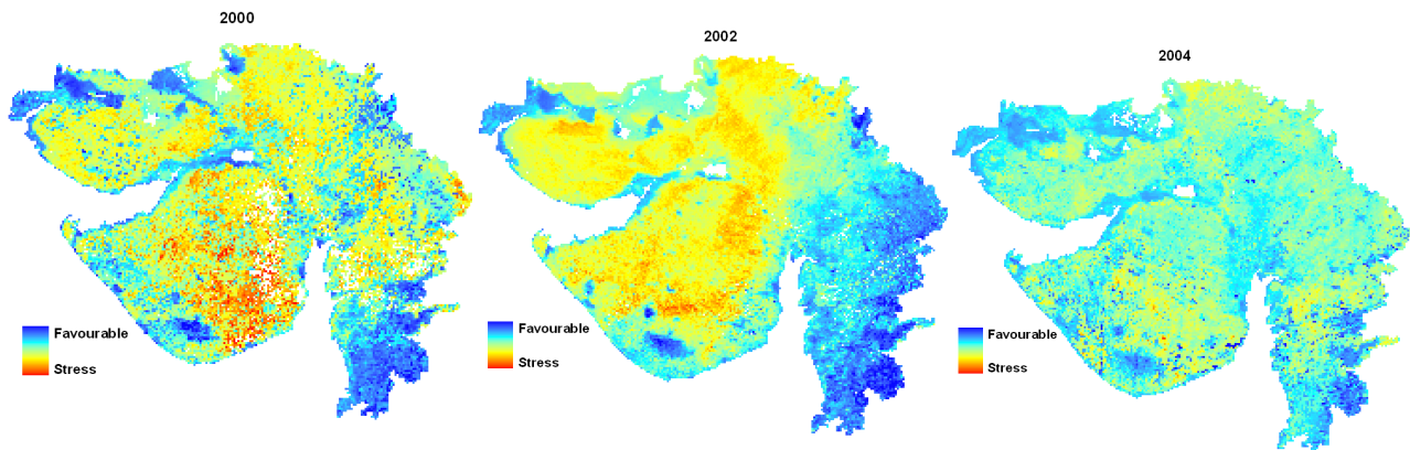
Figure 5.3: Spatial pattern of VTCI on 249 JD during 2000, 2002 and 2004 in Gujarat state
