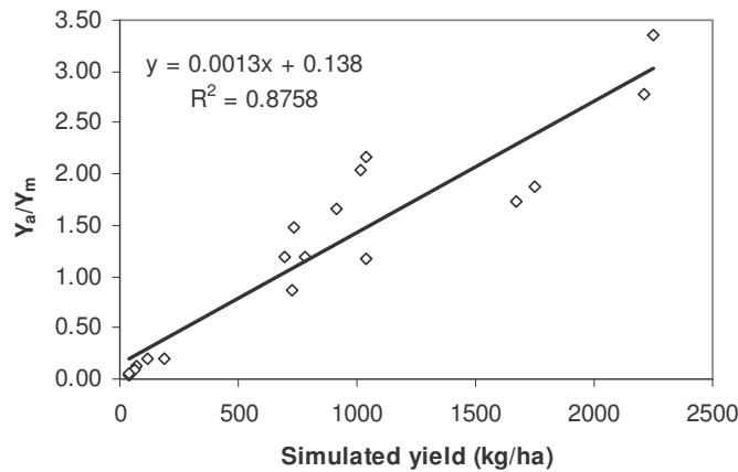
Figure 5.19: The relationships between simulated yield and yield departure
