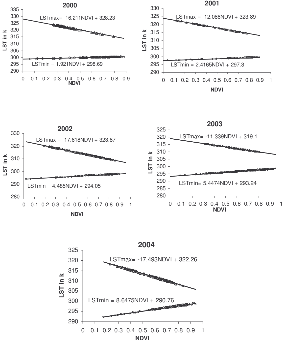
Figure 5.1: The warm edge and cold edge from NDVI-Ts space on 257JD
