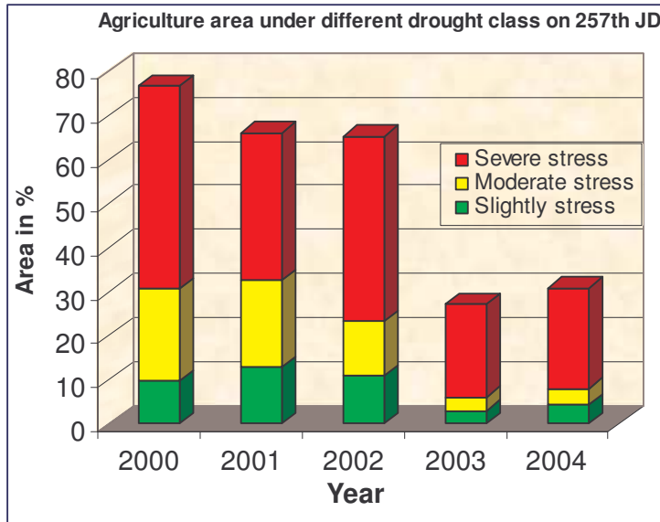
Figure 5.14: The agriculture area under different drought stress on 257 th JD
