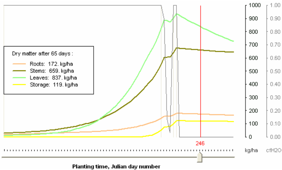
Figure 5.17: The coefficient of water sufficiency index (cfH2O) and dry matter growth curves simulated from PS-n model for Rajkot, 2002
