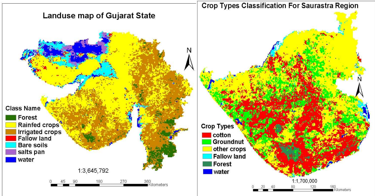
Figure 4.10: The classified land use map and crop types map
