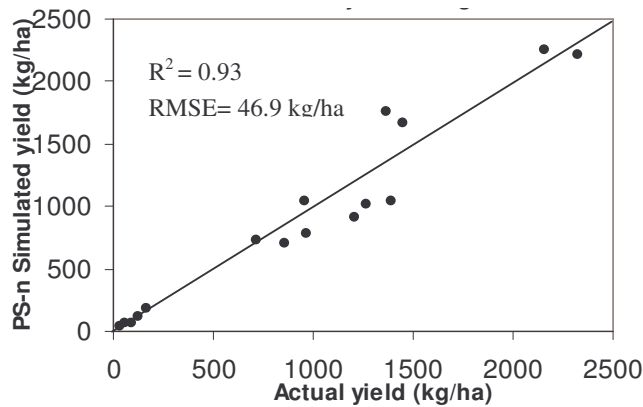
Figure 5.18: 1:1 line comparison between the actual yield and simulated yield of groundnut
