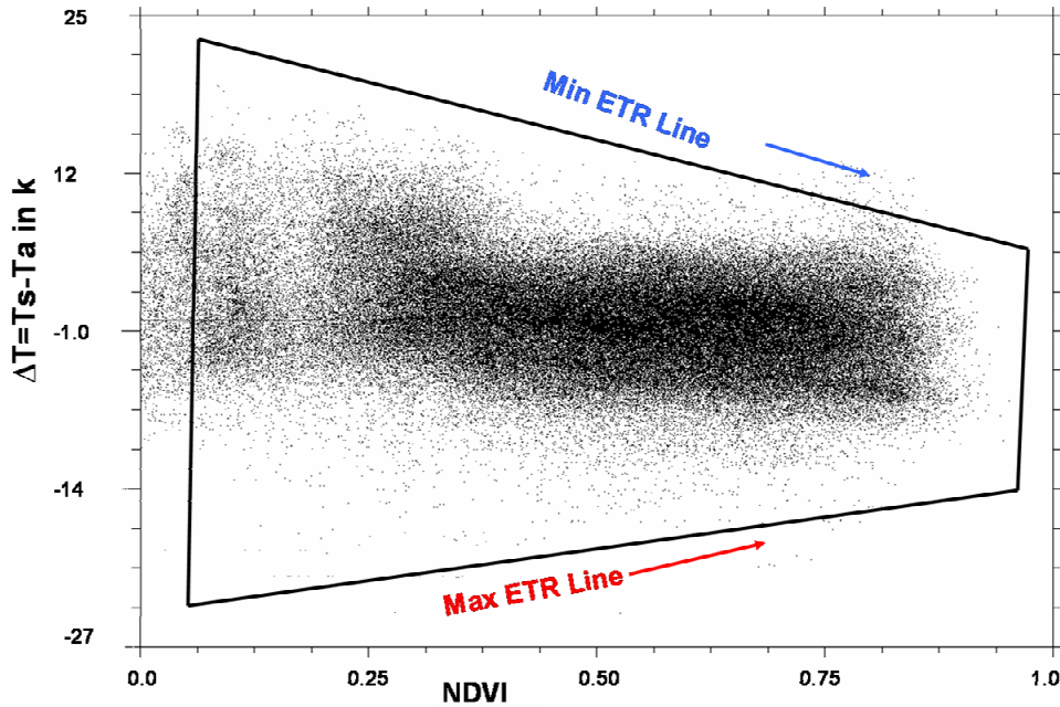
Figure 4.8: Schematic scatter plot of physical interpretation of WDI based on NDVI- \Delta T space
