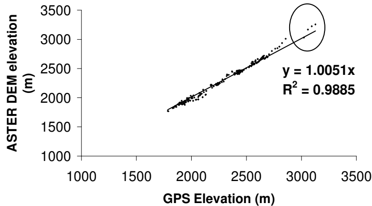
Figure 15 Correlation of points from Raw ASTER DEM and GPS points
