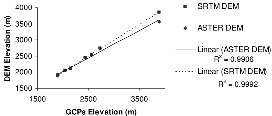
Figure 19 ASTER and SRTM DEMs compared to Tri.GCPs
