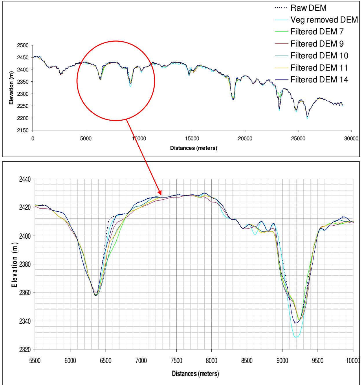
Figure 23 Profile of the raw SRTM DEM and DTMs selected for qualitative assessment
