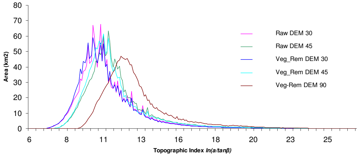
Figure 39 Topographic Index- Area distribution in Malewa catchment for different resolution SRTM raw DEM and Ilwis DTM
