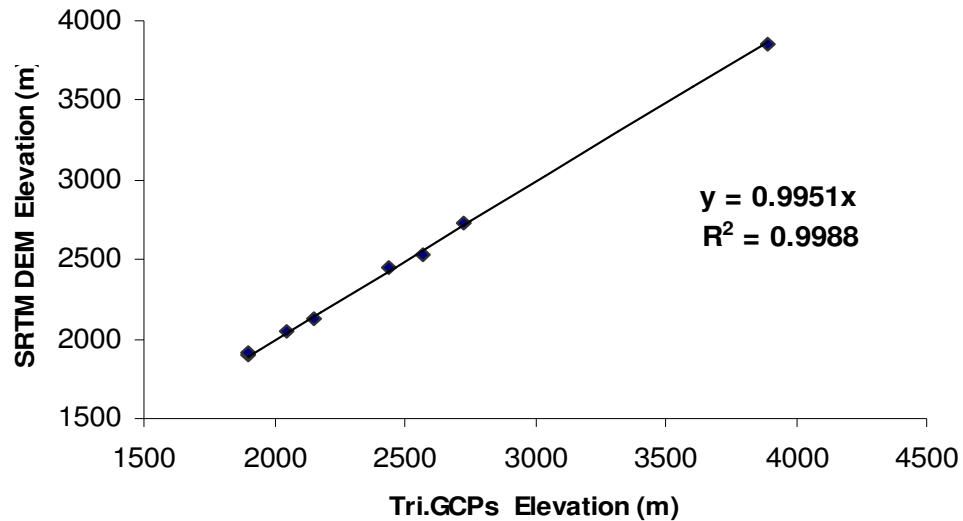
Figure 12 Correlation of points from Raw SRTM DEM and Tr.GCPs
