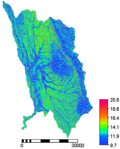
Figure 37 Topographic Index map of Malewa Basin extracted from the raw SRTM DEM
