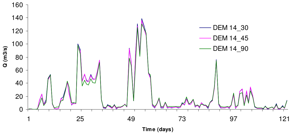
Figure 35 SWAT Model runoff output of Malewa River for filtered and resampled SRTM DTMs of 30m, 45m, and 90m resolutions
