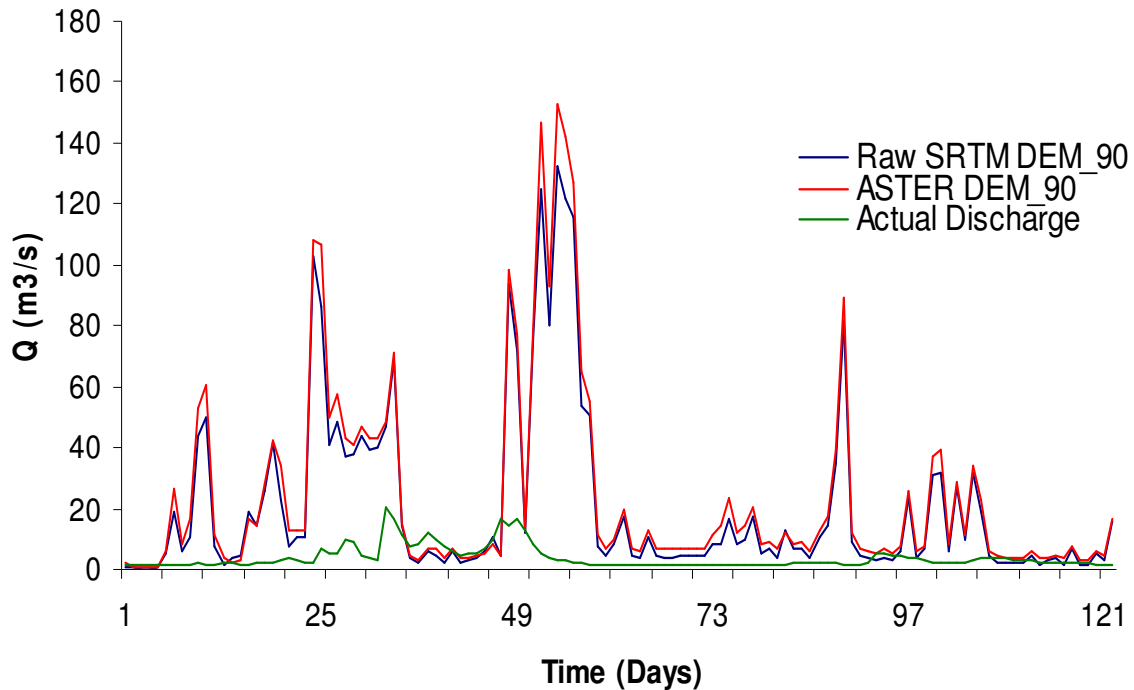
Figure 33 SWAT daily runoff output of Malewa basin for raw SRTM and ASTER DEMs.
