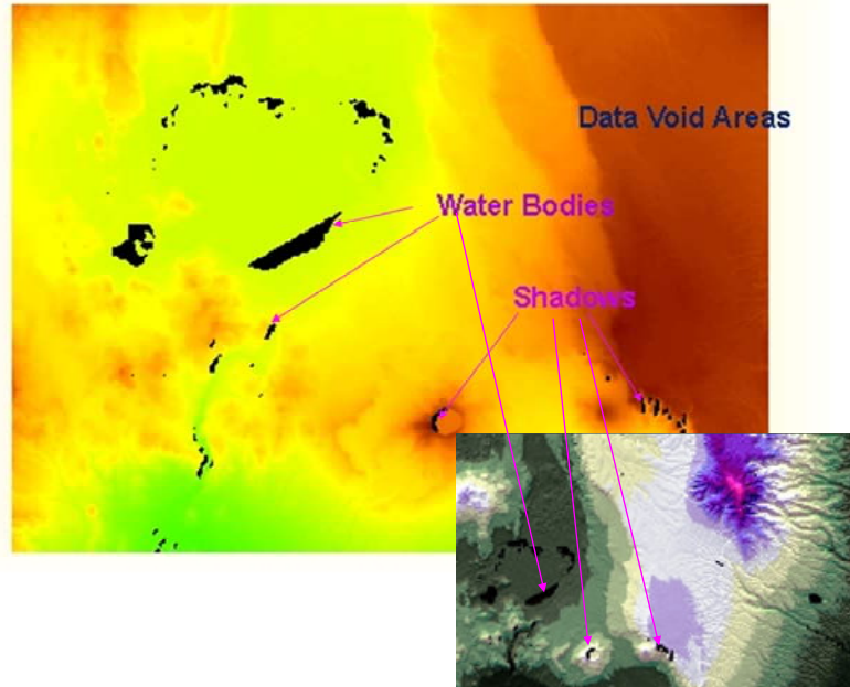
Figure 10 Data voids in raw SRTM DEM of Naivasha basin
