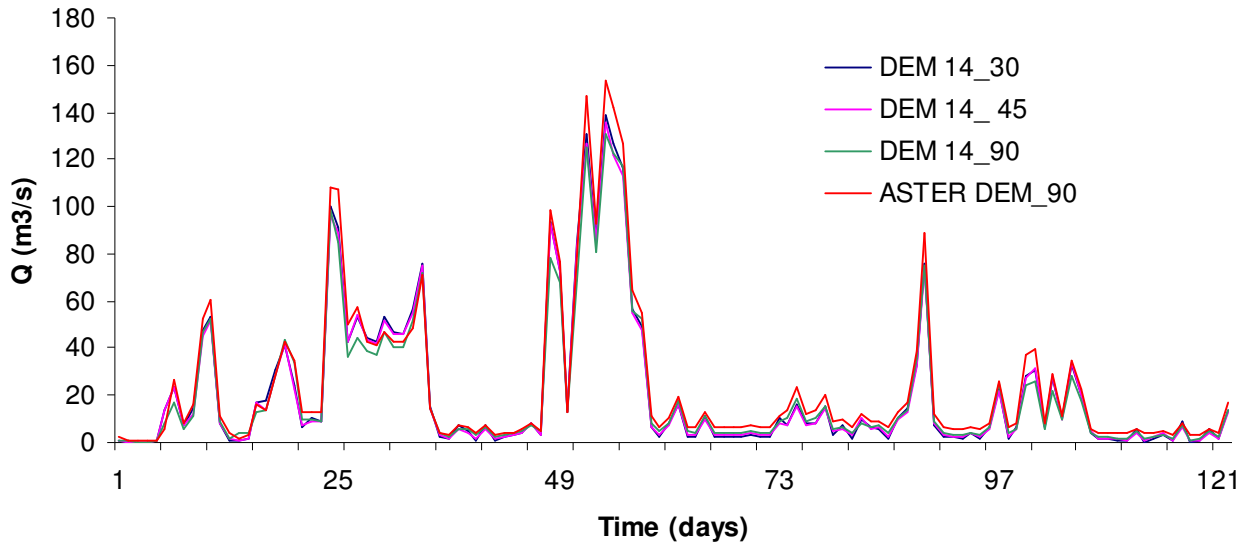
Figure 36 SWAT Model runoff output of Malewa basin for filtered and resampled SRTM DTMs and ASTER DEM
