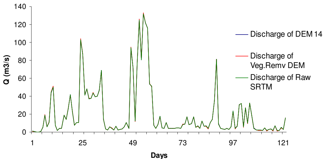
Figure 34 SWAT Model Runoff output of Malewa River for improved and Original SRTM DEMs
