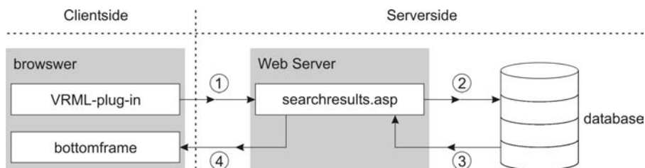
Figure 8.7: Model of the architecture of the prototype.
