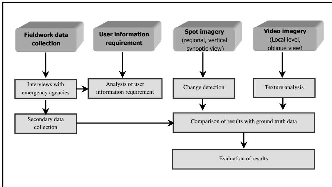
Figure 1.7. Study design
