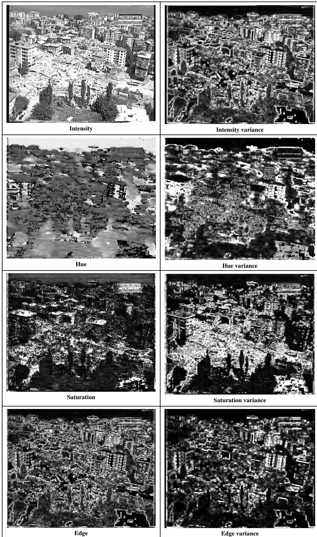
Figure 7.8. Feature layers
